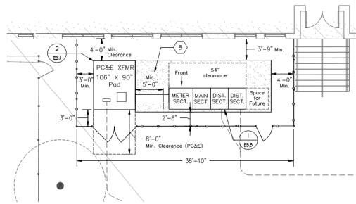
2 Electrical Switchgear Dimensions
